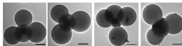
Figure 2. A time series of TEM images showing the growth of the silica core of tetrapods. From left to right, time after the beginning of the addition of 100 µL of TEOS is: 0 min, 30 min, 60 min, and 240 min. Scale bar: 100 nm.
